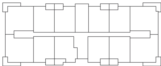
Floors Two-Four
